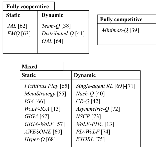
Fig. 1. Breakdown of MARL algorithms by the type of task they address.
