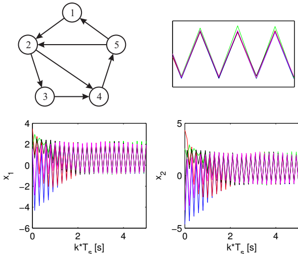
Fig. 3. Consensus of Hammerstein systems. Top-left: Communication graph. Bottom: State trajectories (the sampling time is taken 0.1s). Top-right: zoom-in on the last portion of the x_2 trajectory; note the agents are synchronized.
