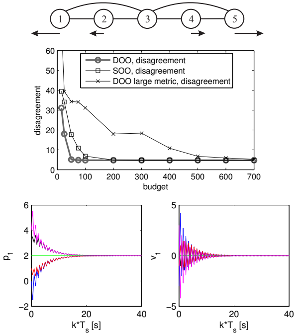
Fig. 2. Top: Connection graph for double integrators, with initial velocities symbolized by arrows. Middle: Results for varying N . Bottom: A representative trajectory.
