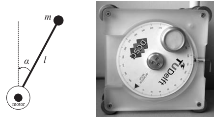
Fig. 1. Inverted pendulum schematic (left) and the real system (right).
